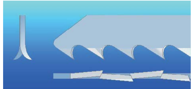
Ground and side set teeth
